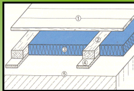
Floor insulation
