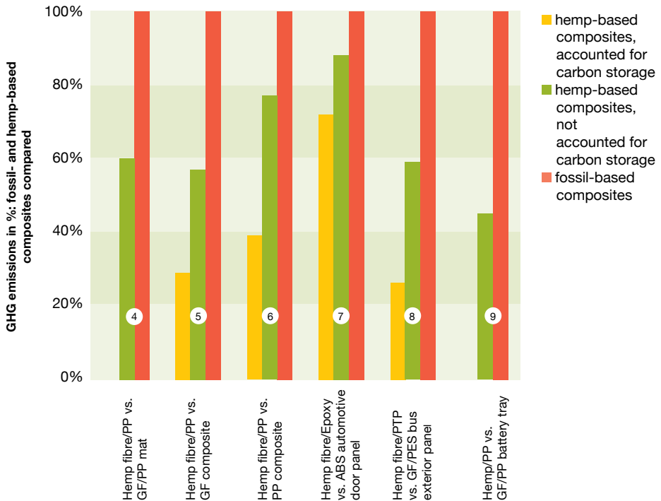
Figure 16: GHG emissions expressed in percent for the production of fossil based and hemp based composites for a number of studies – showing the effects of biogenic carbon storage where available (Haufe & Carus 2011)
