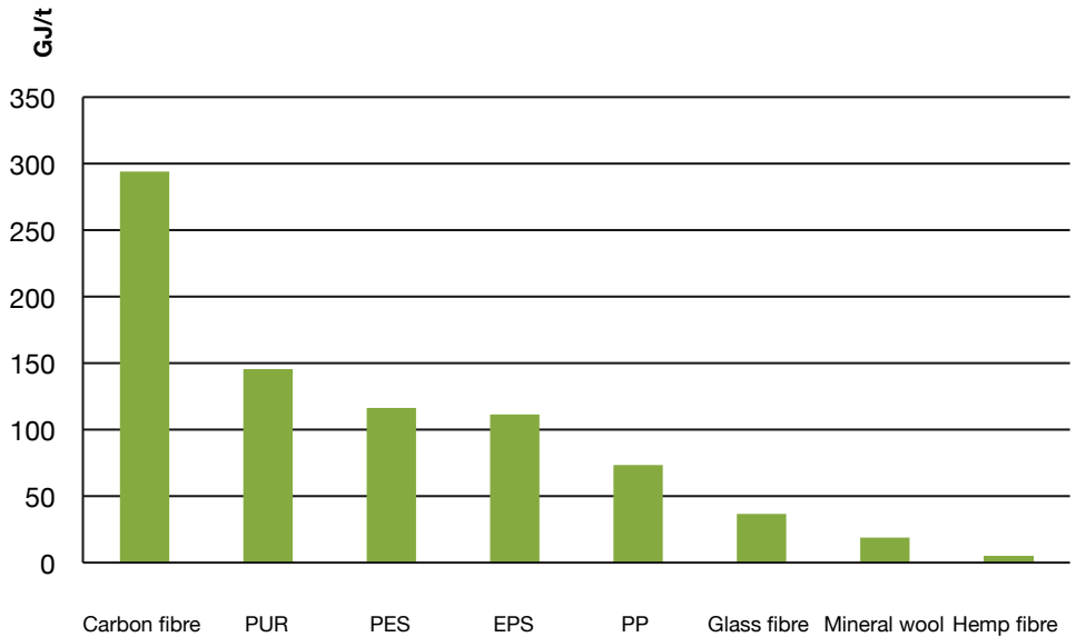
Figure 15: Primary energy use of different materials in GJ/t (Haufe & Carus 2011)
